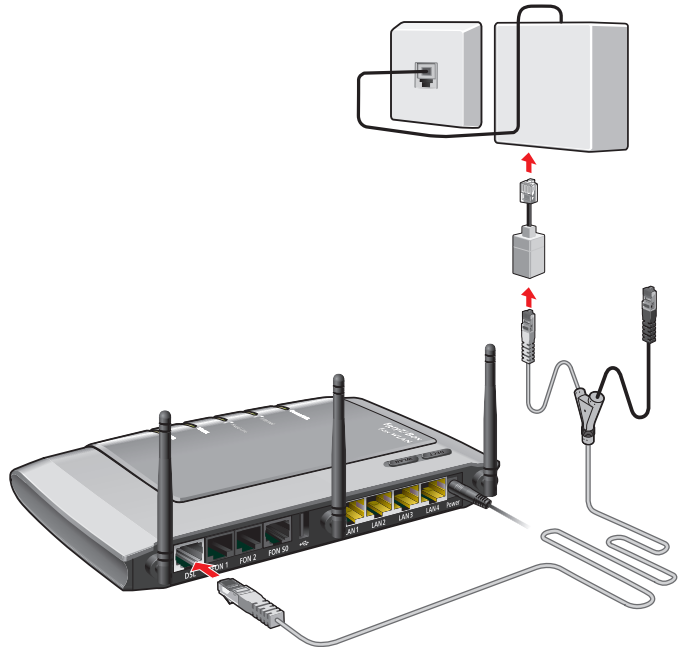
Connecting to the DSL splitter
