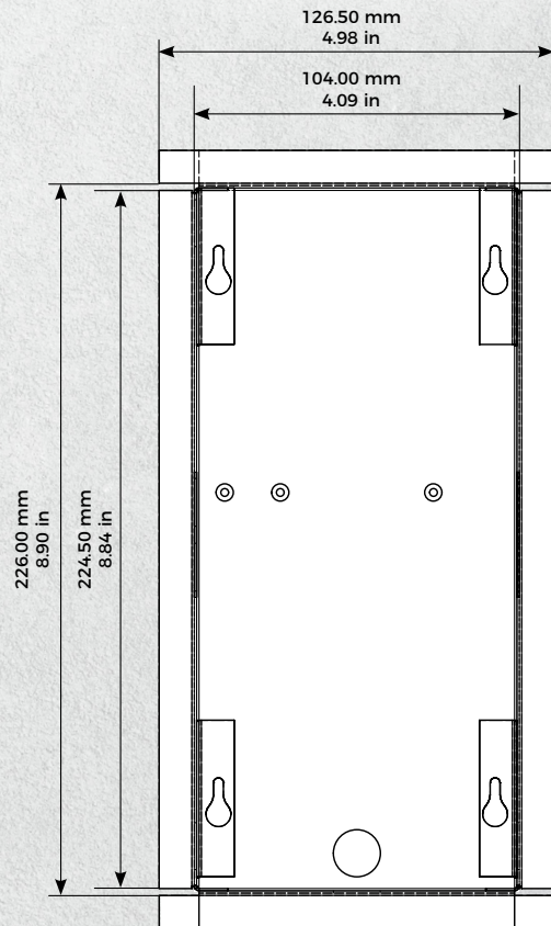
Mounting housing
