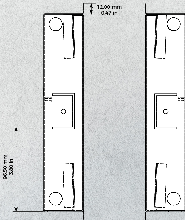
Mounting housing
