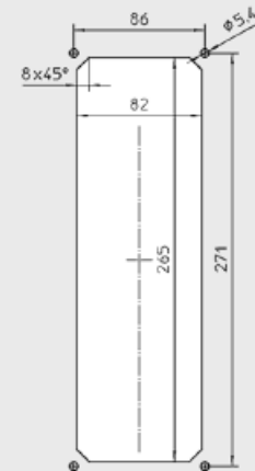
Mounting opening
