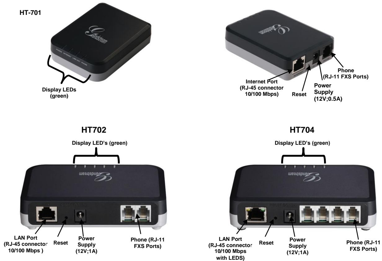
FIGURE 1: DIAGRAM OF HT70X
